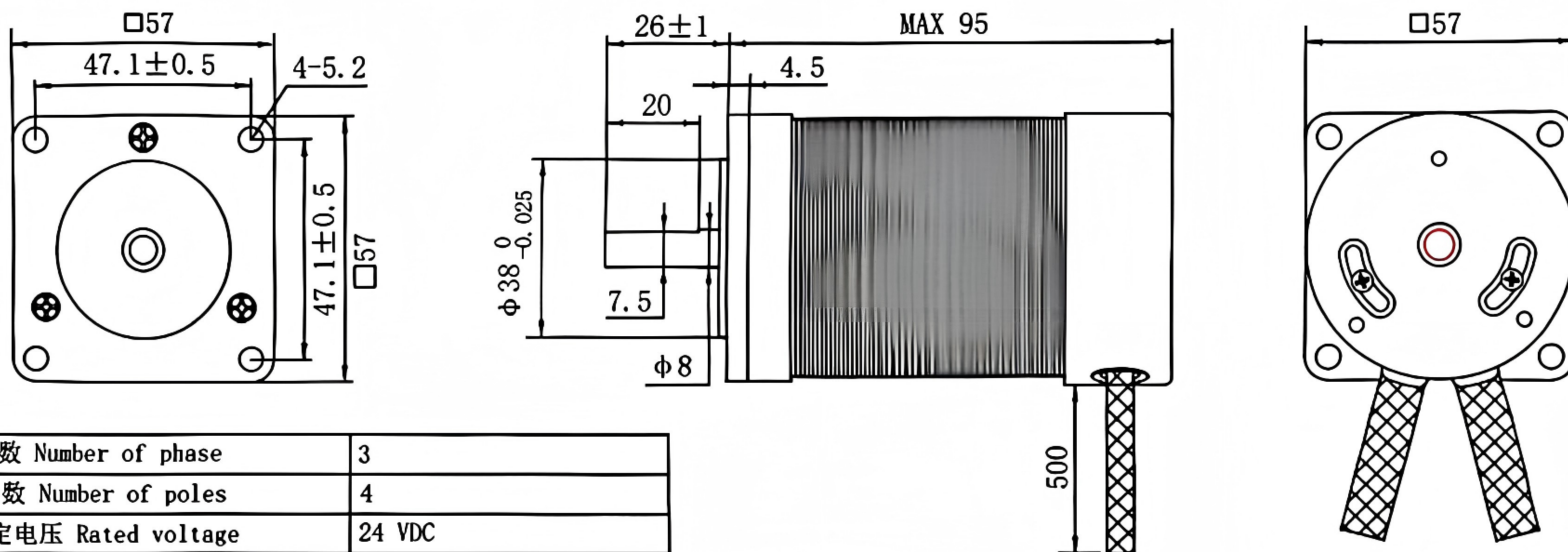
尺寸图 Dimensional drawing
