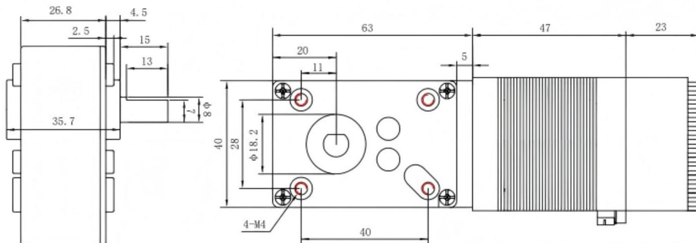
尺寸图 Dimensional drawing
