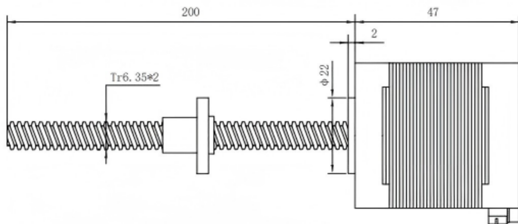
尺寸图 Dimensional drawing
