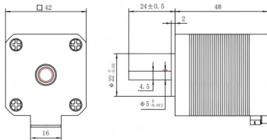
尺寸图 Dimensional drawing
