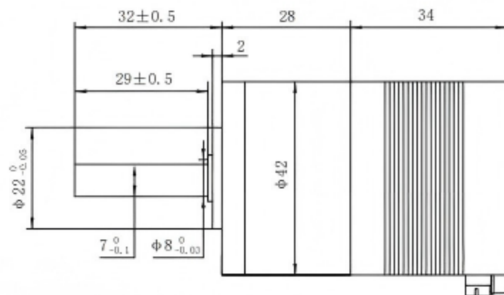
尺寸图 Dimensional drawing
