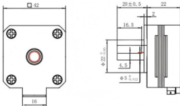
尺寸图 Dimensional drawing
