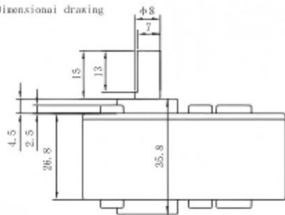
涡轮蜗杆减速机 Turbine worm Reducer
