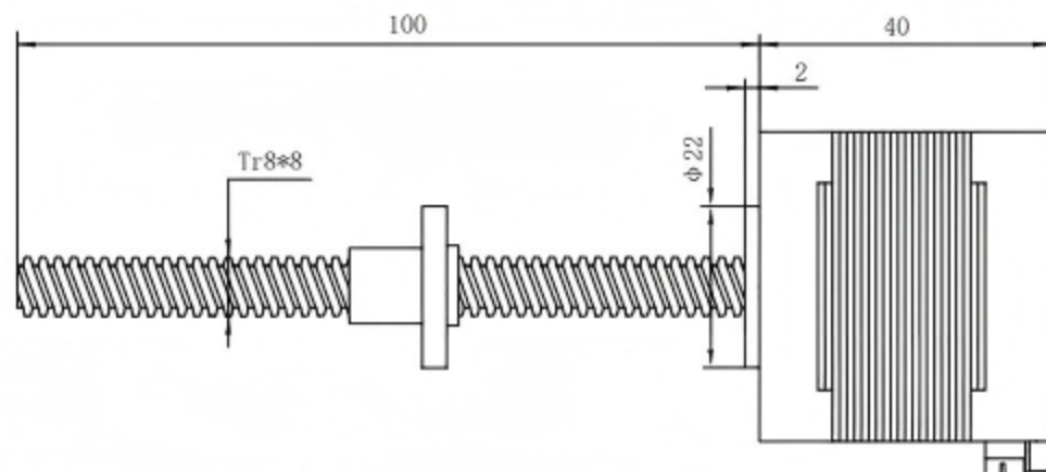
尺寸图 Dimensional drawing
