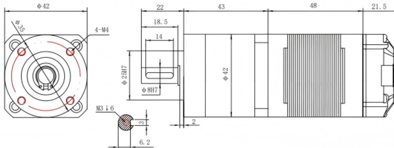
尺寸图 Dimensional drawing
