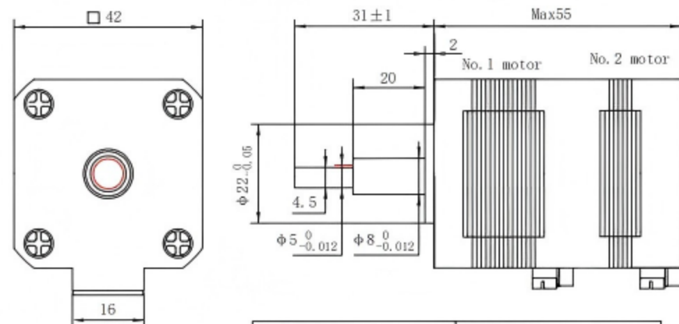
尺寸图 Dimensional drawing
