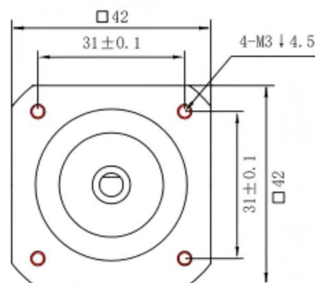
尺寸图 Dimensional drawing
