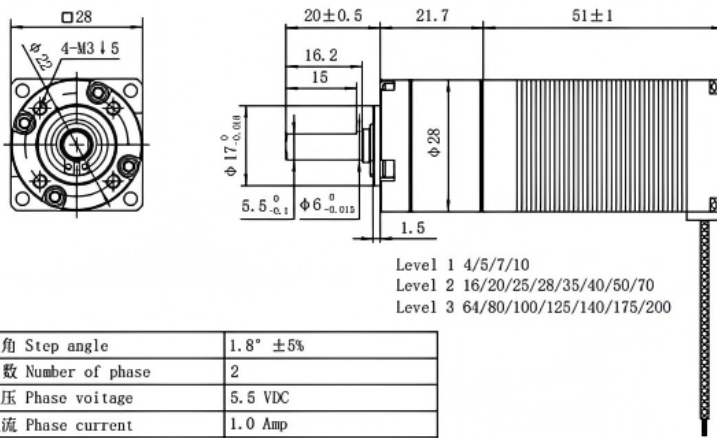
尺寸图 Dimensional drawing
