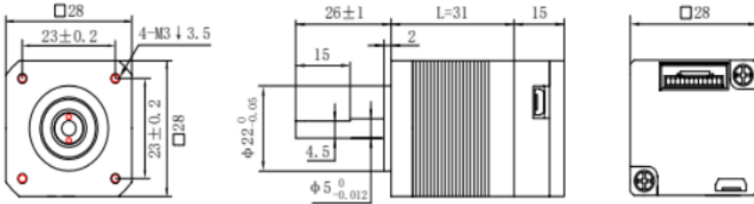
尺寸图 Dimensional drawing
