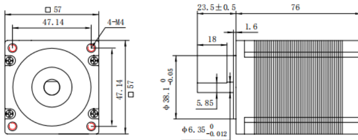
尺寸图 Dimensional drawing
