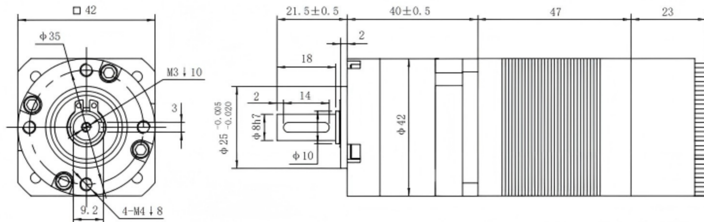
尺寸图 Dimensional drawing
